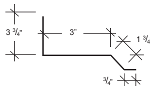
Wall Transition
