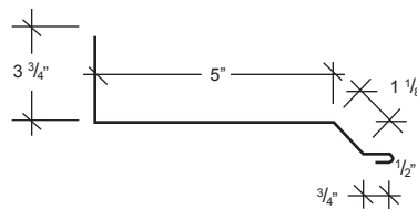
Wall Transition
